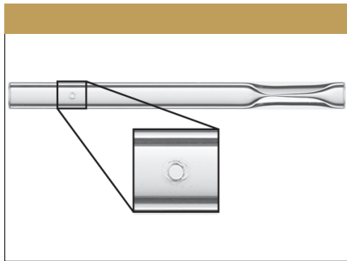
Figure 3: Hole in the wall of a direct injection inlet liner for EPC systems.
